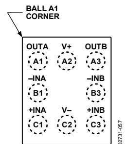
AD8606 TOP VIEW (BALL SIDE DOWN)
